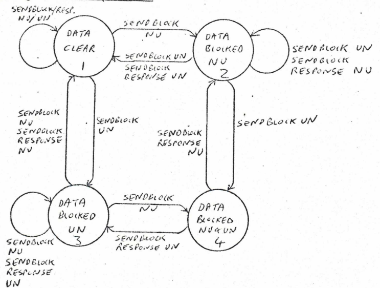
Data Port State Diagram Figure Four
