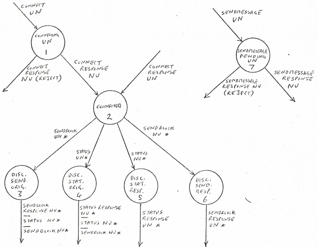
Main Port State Diagram Figure Two
