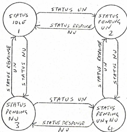
Status Port State Diagram Figure Three
